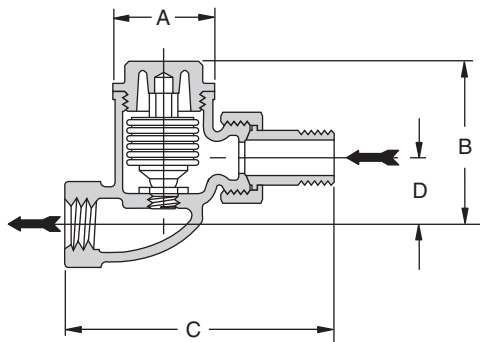
TS-2 Air Vent Straight Type
