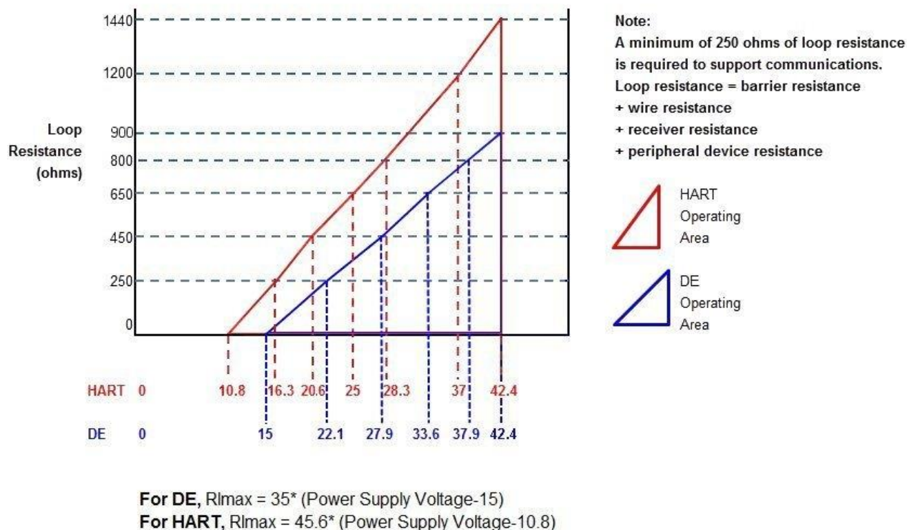
Figure 2 - Supply voltage and loop resistance chart & calculations
